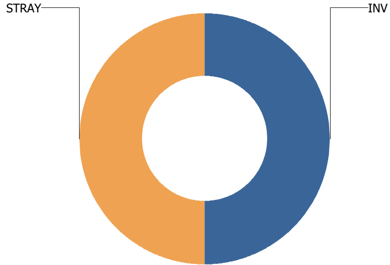
Call Types For SEYMOUR
