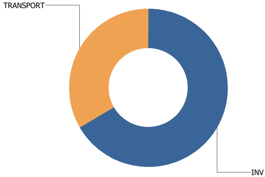
Call Types For SAVOY
