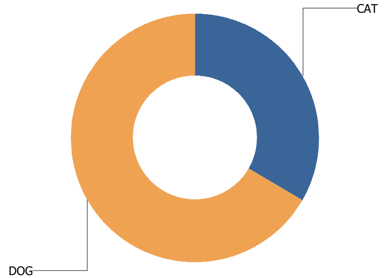
Calls Per Species For SAVOY
